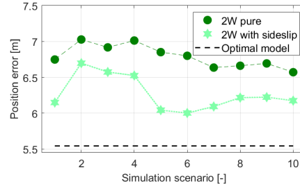
Fig. 9. Position errors of scenarios
