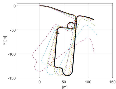
Fig. 1. Odometry paths
