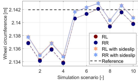
Fig. 8. Wheel circumferences of scenarios
