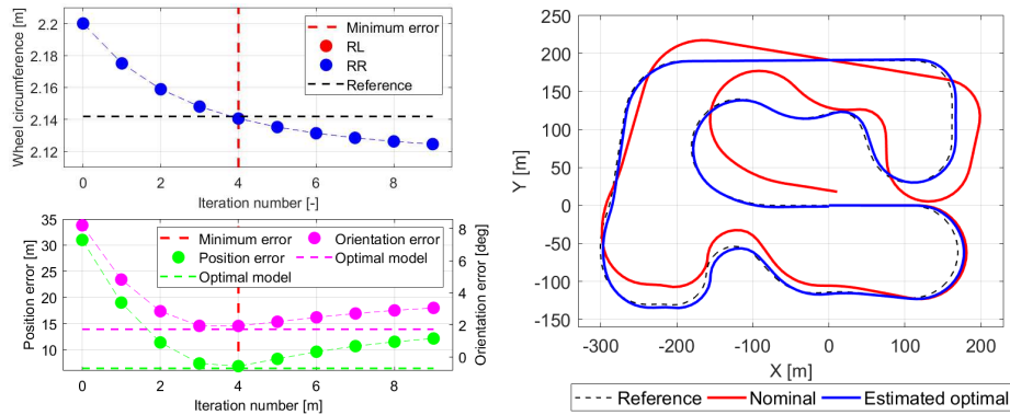
Fig. 6. Results of iteration in Scenario 5. Fig. 7. Track of estimation in Scenario 5.
