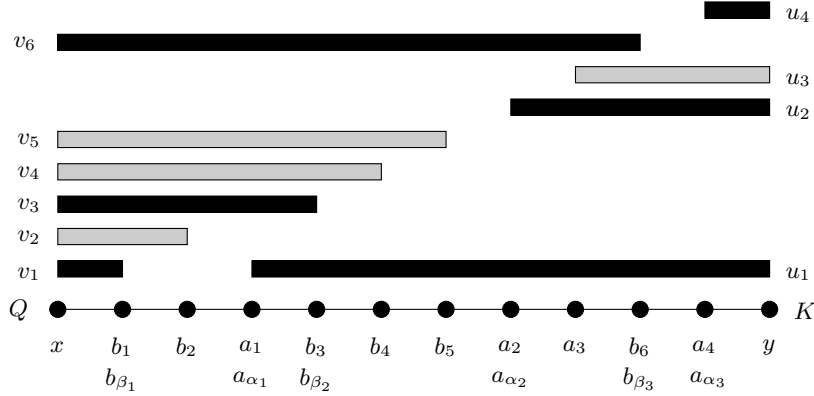
Fig. 5. Proof of Lemma 14: the path between nodes x and y . The rectangles show the subtrees of the v_i 's and u_i 's on this path.
