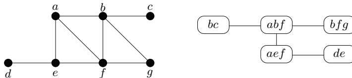
Fig. 1. A chordal graph and its clique tree decomposition.
