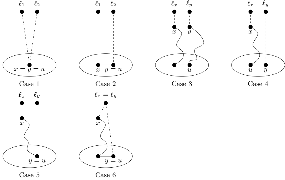
Fig. 7. The cases in the proof of Lemma 19.
