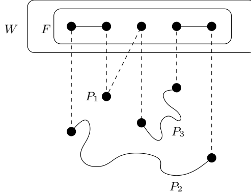
Fig. 6. The fragments F , P_1 , P_2 , P_3 of a hole.
