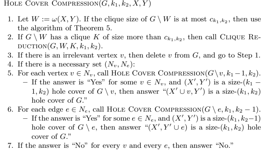
Fig. 3. Algorithm HOLE COVER COMPRESSION.
