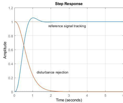
Figure 16: Unit step reference signal tracking and disturbance rejection of the YOULA parameterized controller
