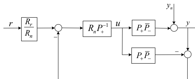
Figure 11: IMC form of YOULA parameterization with filters
