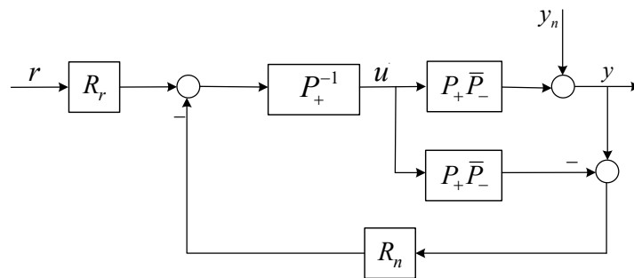
Figure 10: IMC form of YOULA parameterization with reference and disturbance filters
