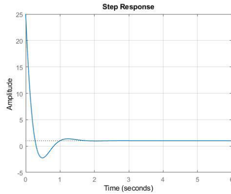
Figure 15. Control signal in case of pole cancellation
