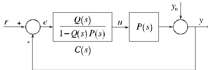
Figure 8: YOULA-parametrized closed-loop
