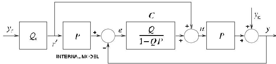
Figure 12: Two-degree-of-freedom version of the YP control loop
