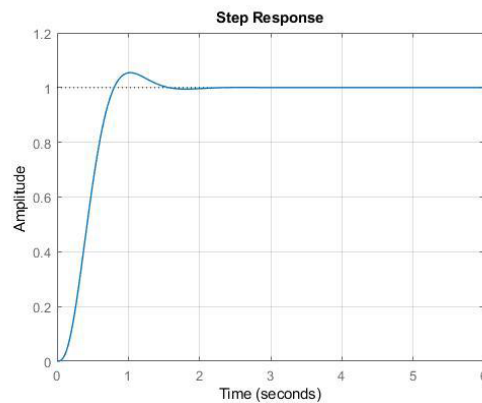
Figure 14. Step response with pole cancellation
