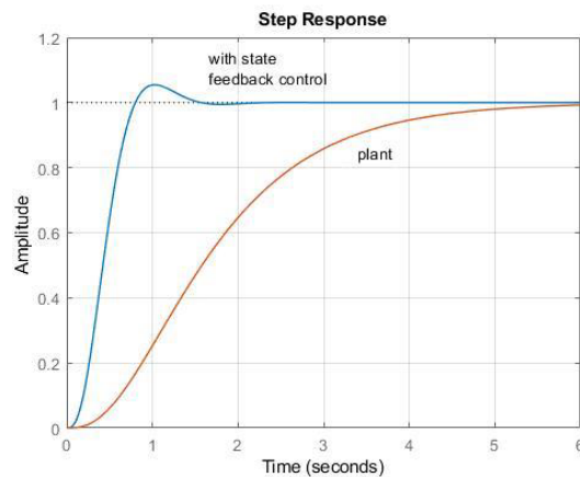
Figure 13. Step response with state feedback control
