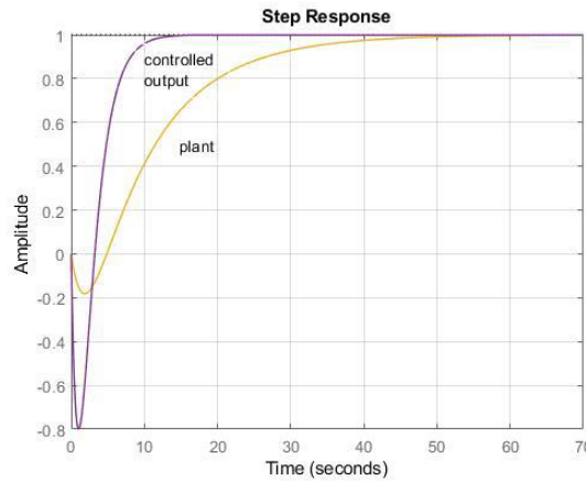
Figure 17: YOULA control of a non-minimum phase plant
