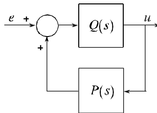
Figure 7: Realization of a YP regulator
