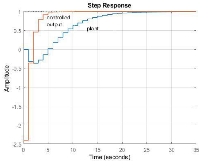
Figure 18. Unit step responses of the plant and the controlled system
