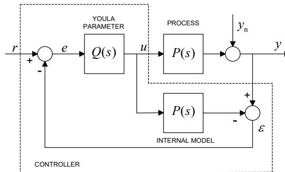
Figure 9: IMC form of YOULA parameterization
