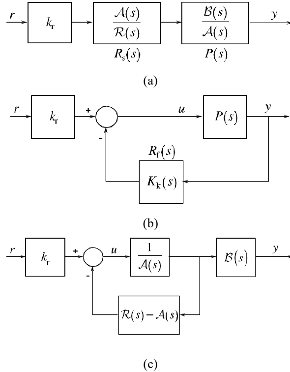
Figure 2: Equivalent schemes to the state feedback design using transfer functions and polynomials
