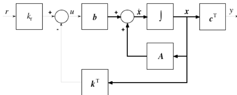
Figure 1: Linear regulator with state feedback
