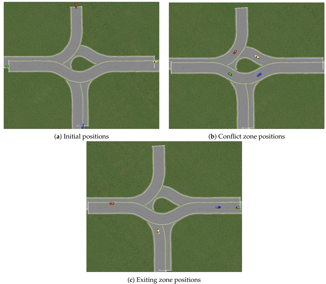
Figure 7. AVs motion in the roundabout using MPC control.
