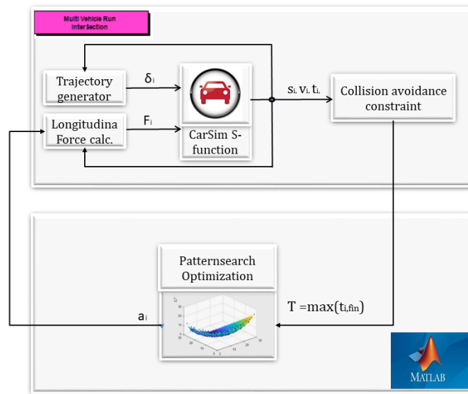
Figure 9. Offline time-optimal optimization in CarSim environment.
