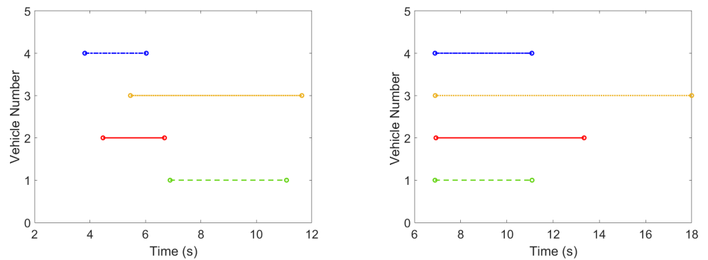
(a) Conflict zone times with minimal traveling time (b) Conflict zone times applying collision avoidance
