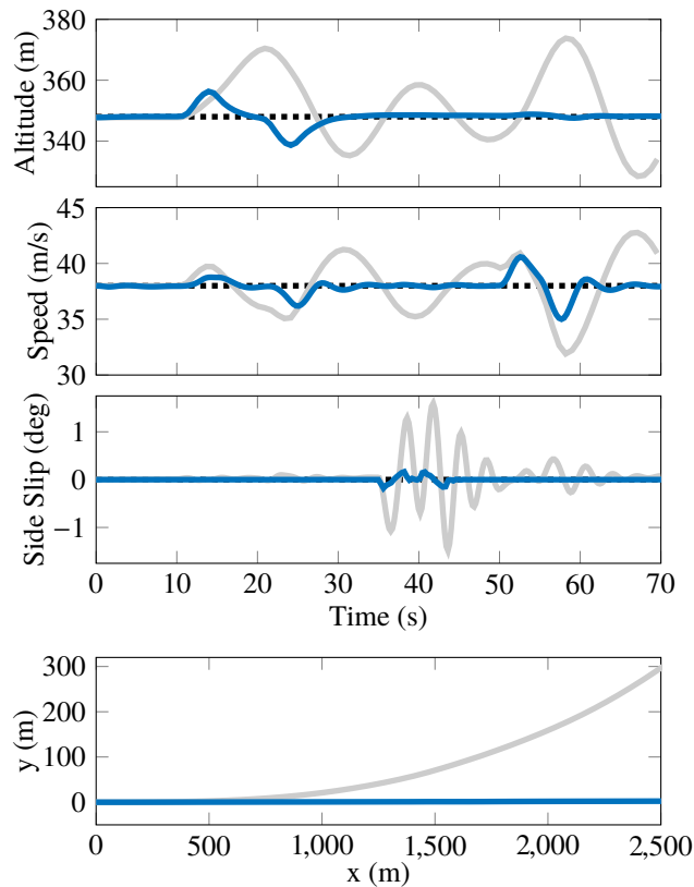
Fig. 12 Gust simulation comparing the open (—) and closed loop (—) results to the reference signals (····) for the controlled variables and aircraft position.
