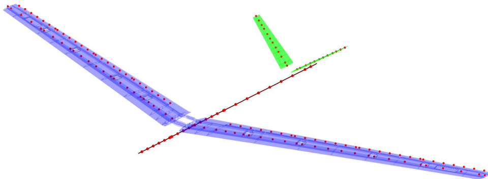
Fig. 4 Full FE model with condensation points [5]
