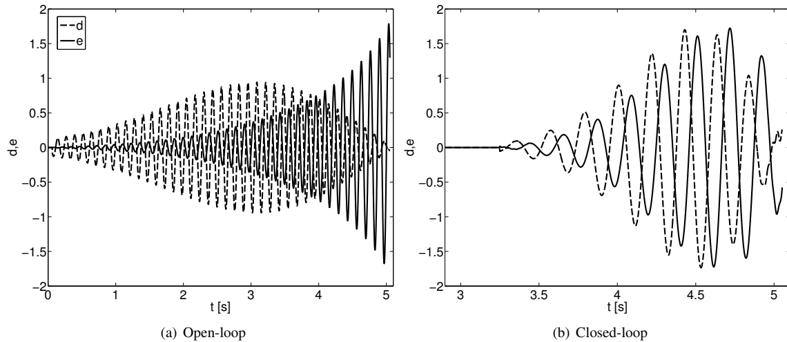
Fig. 31 Worst-case disturbance ( d ) and corresponding wing tip acceleration ( e ) for a trajectory with V_2 larger than the open-loop flutter speed.
