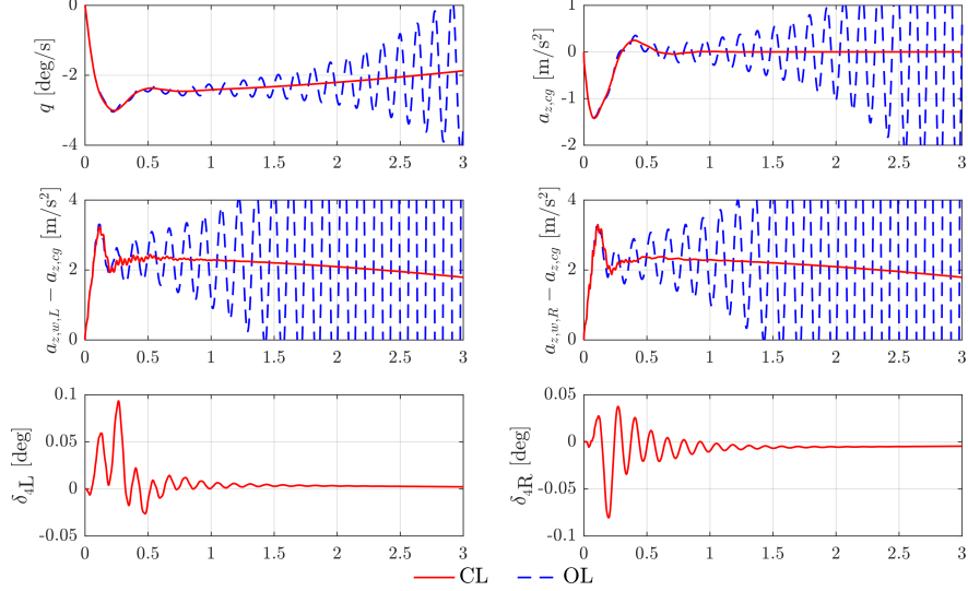
Fig. 28 Response of the closed-loop system with K_s to a step in the elevator \delta_e of the open-loop and closed-loop for N = 10 (below the flutter speed).
