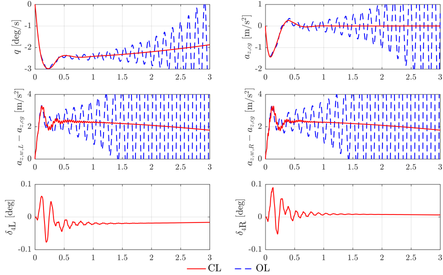
Fig. 25 Response of the closed-loop system with K_r to a step in the elevator \delta_e of the open-loop and closed-loop for N = 10 (above the open-loop flutter speed).
