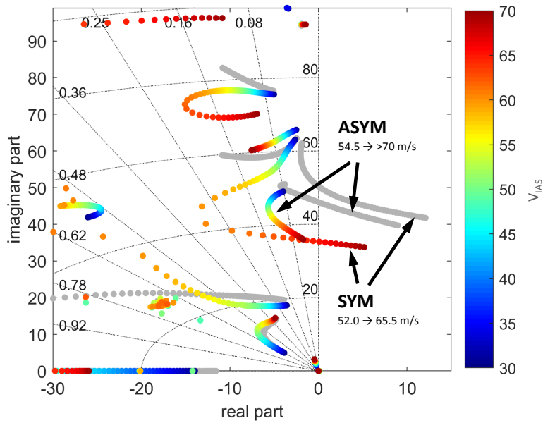
Fig. 18 Comparison of open-loop (gray) and closed-loop poles (colored).
