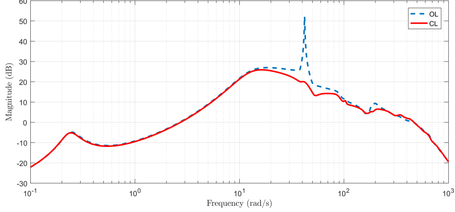
Fig. 24 Maximum singular value of open-loop and closed-loop systems at the speed chosen for synthesis ( N = 13 ) between the inputs \delta_{4L} and \delta_{4R} and the performance outputs \dot{\eta}_1 and \dot{\eta}_2 .
