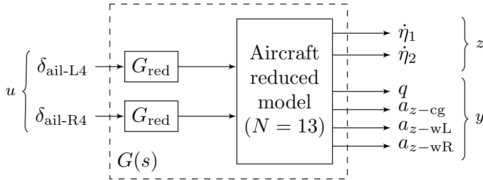
Fig. 21 Synthesis model for H_\infty control design.
