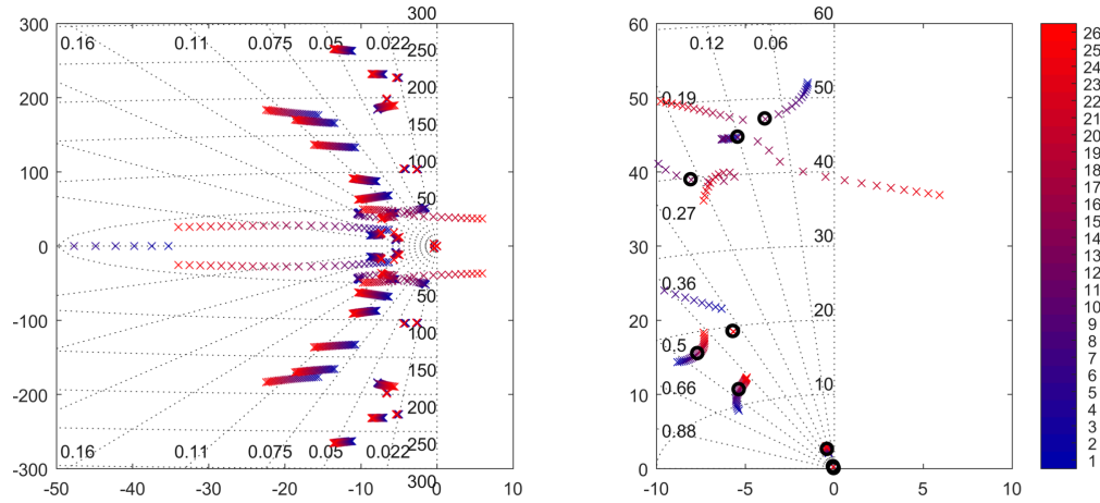
Fig. 26 Pole-zero map of the fifth order Padé approximation of the reduced-order closed-loop system using the structured H_\infty controller, with emphasis on the poles at the synthesis configuration ( N = 13 , V_{TAS} = 57 m/s)
