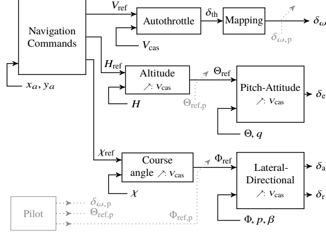
Fig. 7 Control architecture for fully automated flight (mode (iii)), and augmented flight (mode (ii)), indicated in gray.
