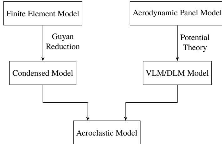
Fig. 3 Modeling process of the demonstrator aircraft
