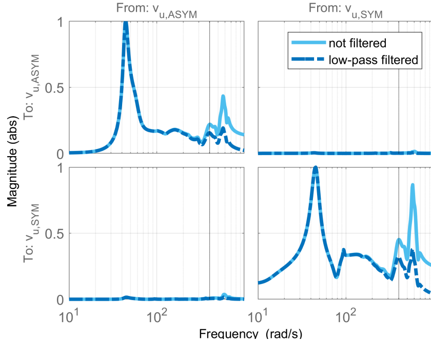
Fig. 16 Transfer functions from blended inputs to blended outputs indicating a good modal decoupling at V_{ias} = 20 m/s.
