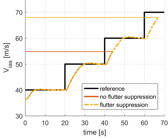
Fig. 19 Increasing aircraft velocity in nonlinear simulation.
