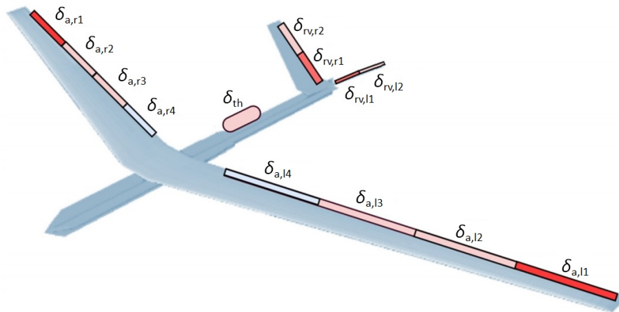
Fig. 2 Control surface configuration.
