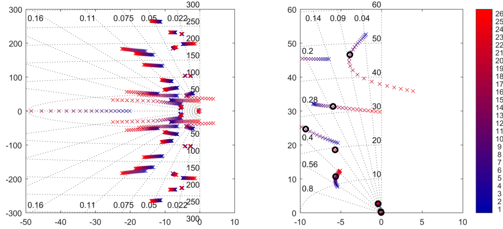
Fig. 23 Pole-zero map of the fifth order Padé approximation of the reduced-order closed-loop system using the reduced controller, with emphasis on the poles at the synthesis configuration ( N = 13 , V_{\text{TAS}} = 57 m/s)
