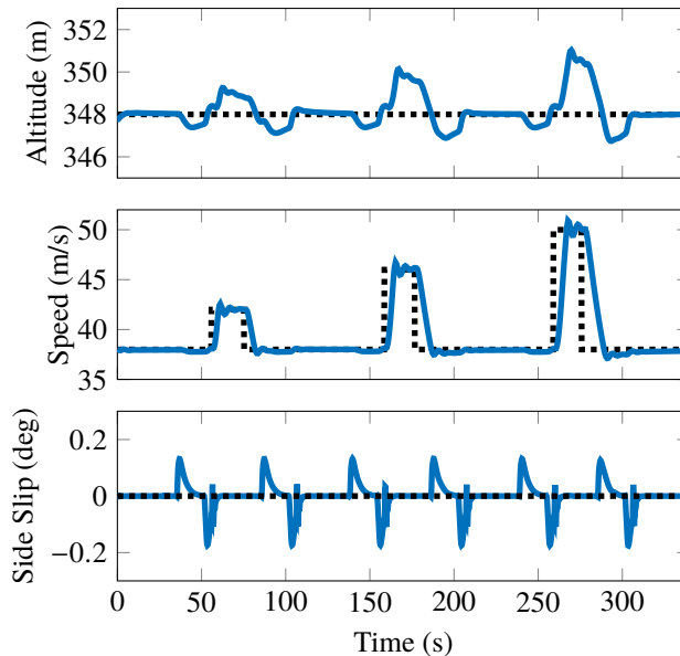
Fig. 10 Closed loop simulation results for the altitude, velocity and side slip angle (—) in comparison to their reference signals (····) during the three lap test pattern
