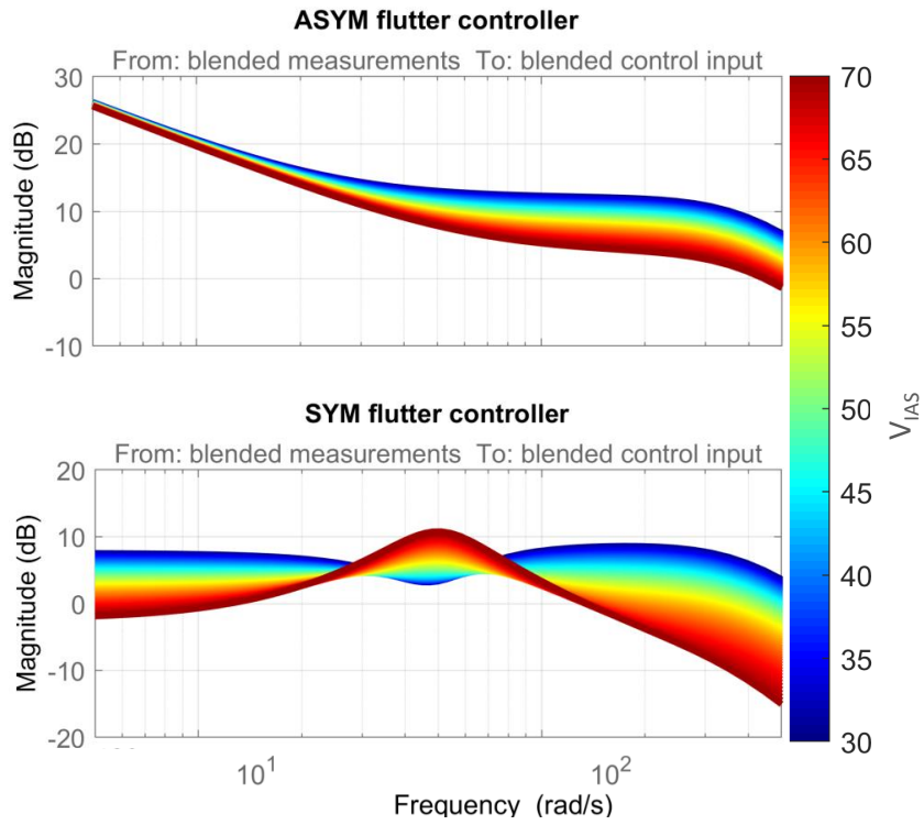
Fig. 17 Gain-scheduled SISO controllers for aeroelastic mode control.
