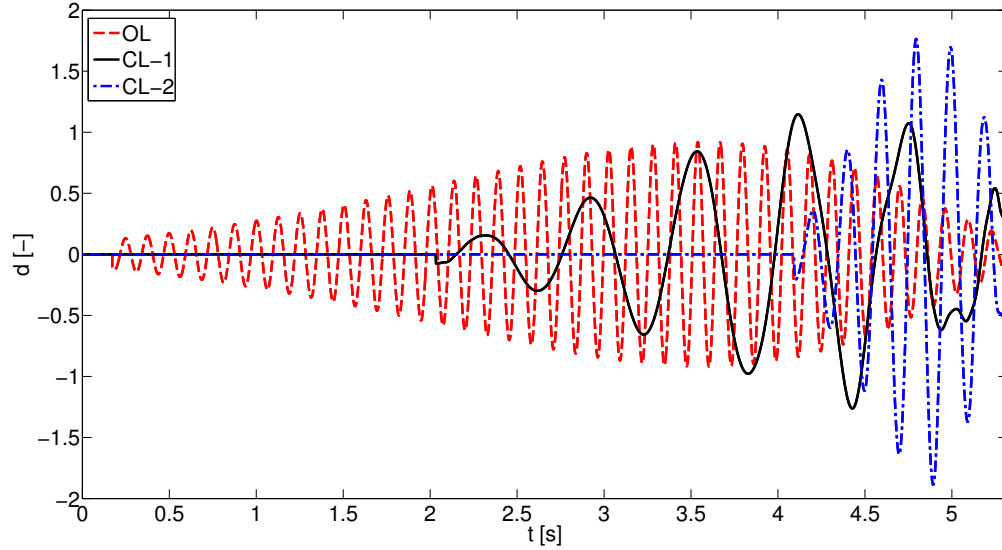
Fig. 29 \mathcal{L}_2 gain worst-case disturbances for a_{z-CG} .
