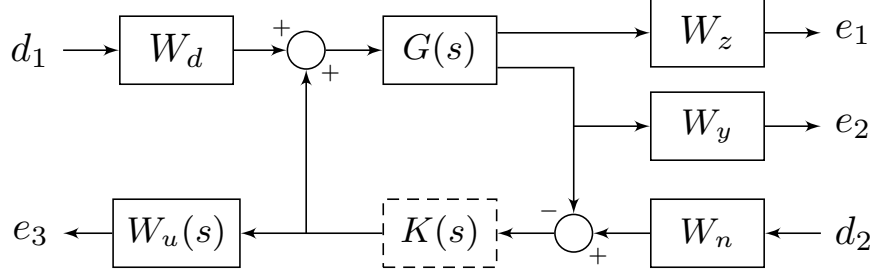
Fig. 22 Generalized plant for H_\infty optimization.
