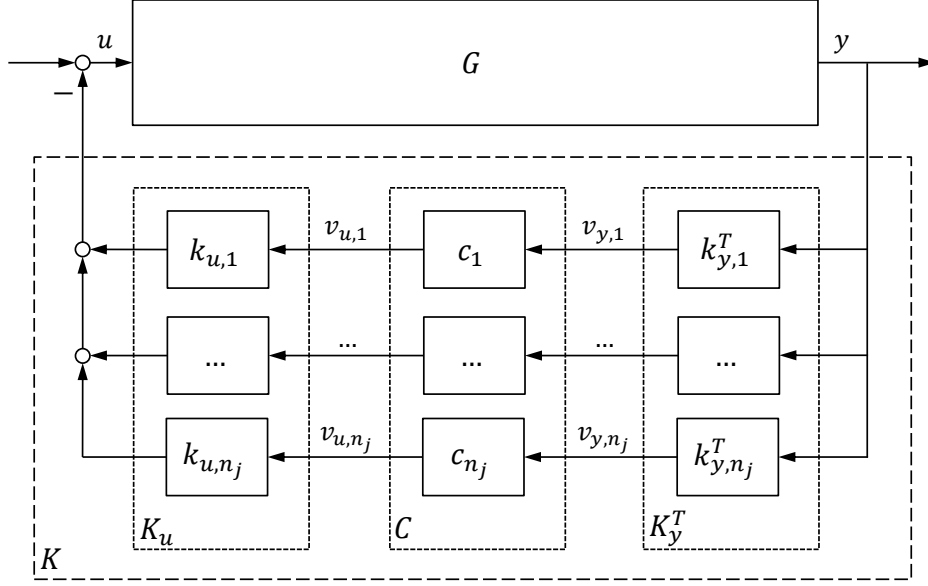
Fig. 14 Closed-loop interconnection of the plant G with the controller K
