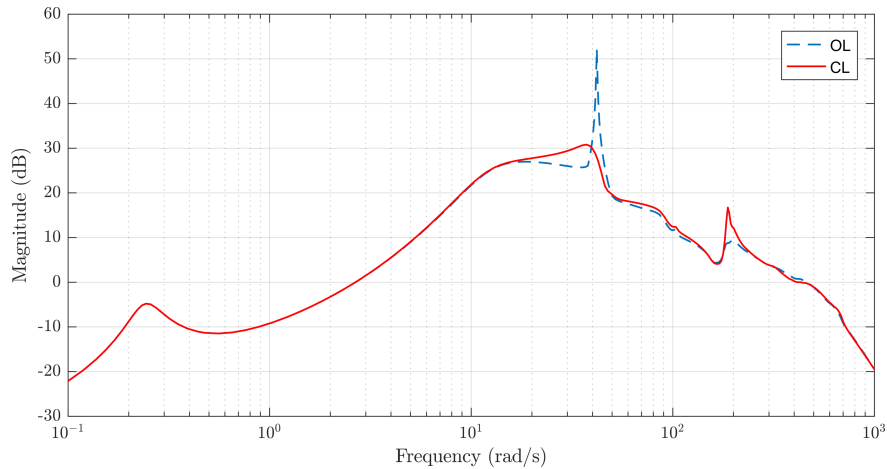
Fig. 27 Maximum singular value of open-loop and closed-loop systems at the speed chosen for synthesis ( N = 13 ) between the inputs \delta_{4L} and \delta_{4R} and the performance outputs \dot{\eta}_1 and \dot{\eta}_2 .
