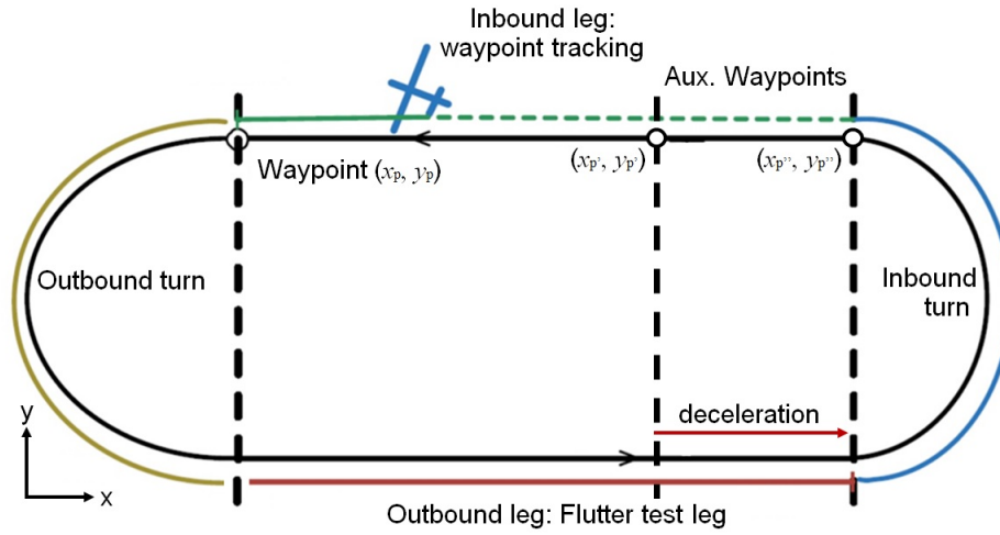
Fig. 8 Flight Test Pattern.
