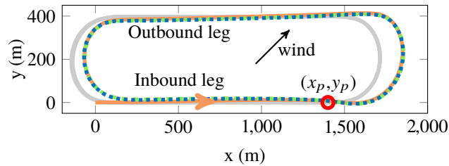
Fig. 11 Simulated flight test pattern with constant wind for lap 1 (—), lap 2 (---), and lap 3 (····) depicted together with the pattern without wind (—).
