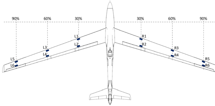
Fig. 20 FLEXOP sensors for flutter control.
