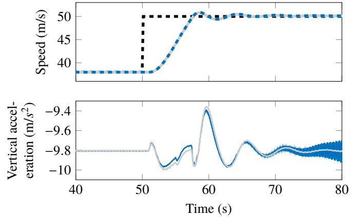
Fig. 13 Speed response (diagram 1) and vertical wing tip acceleration (diagram 2) during an acceleration scenario from 38 m/s to 50 m/s for the flexible (blue) and the rigid (wing set).
