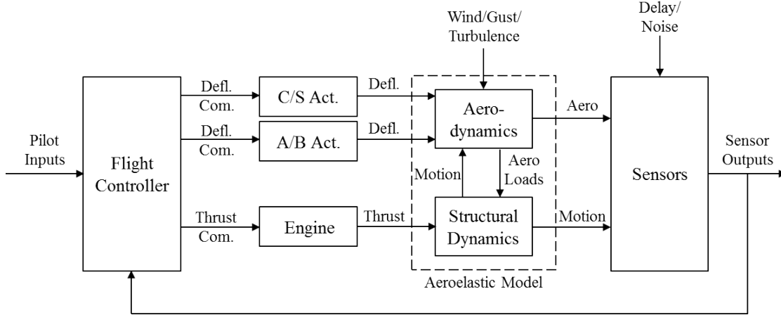
Fig. 6 Aeroservoelastic model [5]
