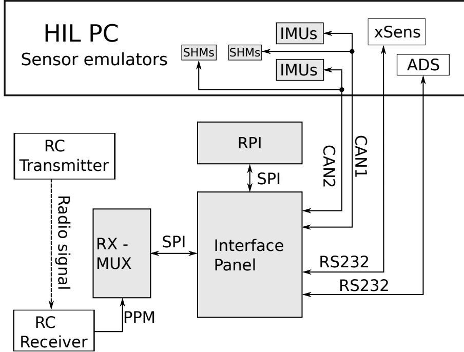
Fig. 32 An over schema of the connection and setup of the HIL developed for the FELXOP demonstrator
