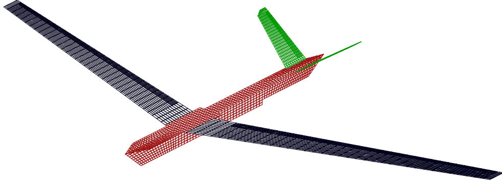
Fig. 5 Aerodynamic boxes of the FLEXOP demonstrator aircraft [5]
