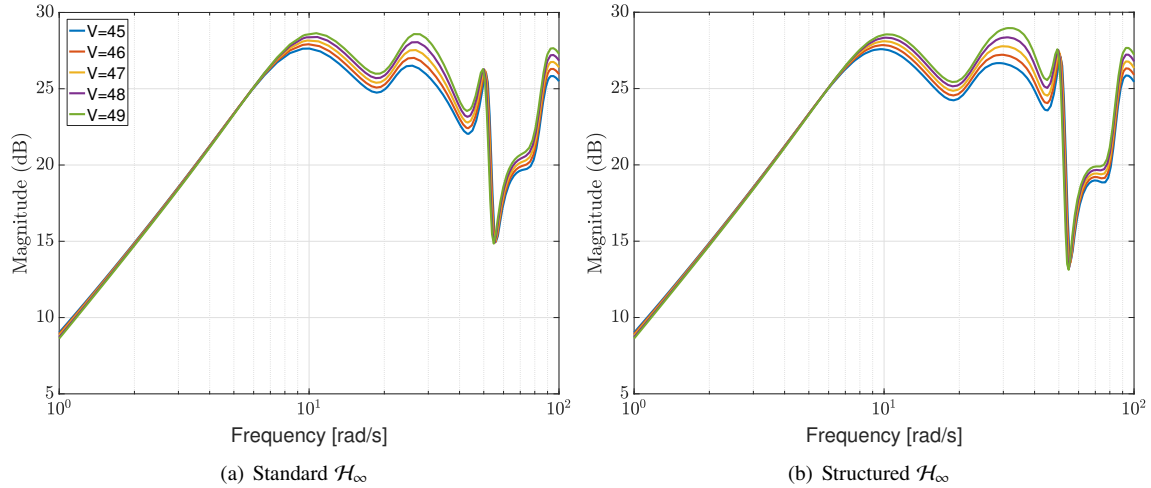
Fig. 30 Bode (magnitude) plot from the gust channel to a_{z-CG} .
