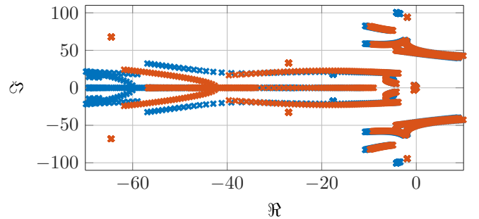
Fig. 6. Pole migration of the LOM (*) and FOM (*)
