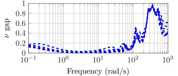
Fig. 5. \nu -gap values between the FOM and LOM
