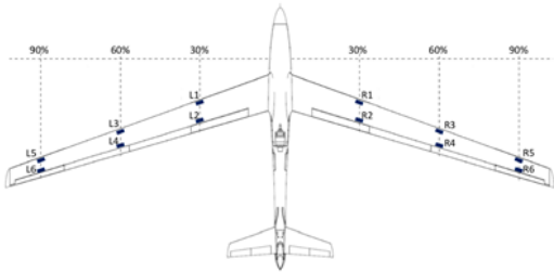
Fig. 3. FLEXOP aircraft sensor configuration
