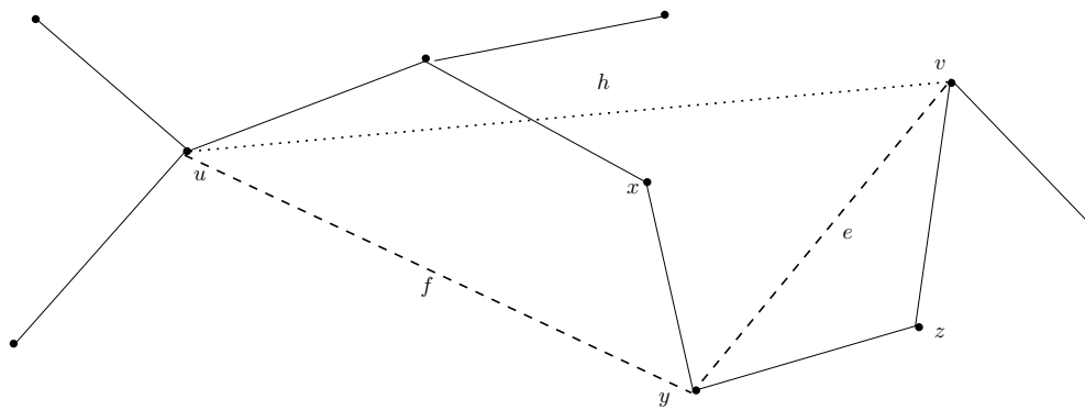
Figure 2: Illustration of Cases I and II in the proof of Theorem 3.6.
