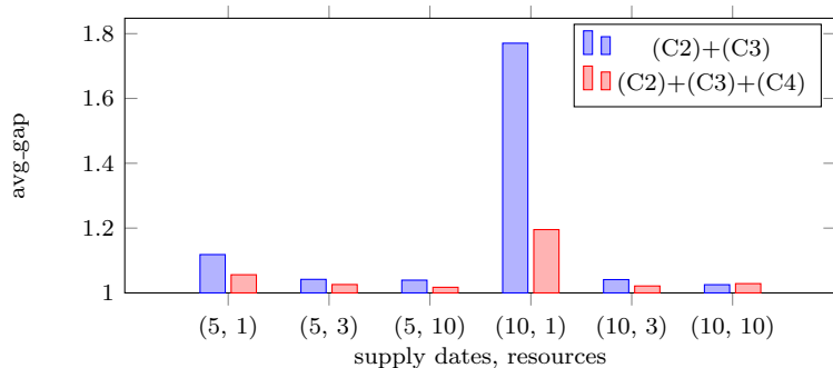
Figure 3: Average gaps in case of 50 jobs. Each bar represents the average over 10 instances.
