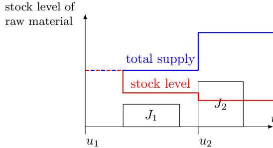
Figure 1: Illustration of the problem. The height of a job indicates the amount of the required raw material.
