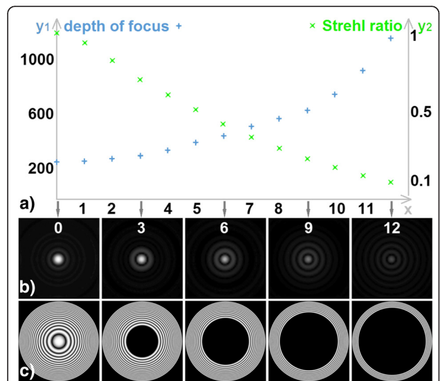
Fig. 5 The effects of the gap-size on the hologram reconstruction properties. a The diagram of the depth of focus (y1, [μm], +) and the Strehl ratio (y2, [-], x) as the functions of the hologram incompleteness. The values of the x-axes denote the number of the missing interference rings. b The reconstructed images of the different gappy holograms, that can be considered also as the spot diagram of the different ring-shaped holograms. c Gappy intensity holograms with different gap-sizes
