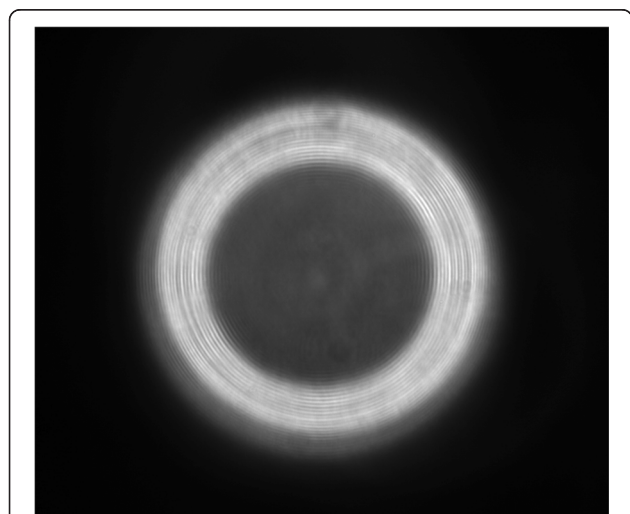
Fig. 4 A typical self-referenced digital intensity hologram using an RBL. Interference fringes only appear in the ring area, due to the geometry of the hollow beam. This results in that the low spatial frequency components will be not recorded in the hologram, and this way they will be missing from the hologram reconstructions too
