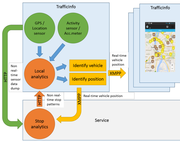
Fig. 6. Sensor data flows in TrafficInfo
