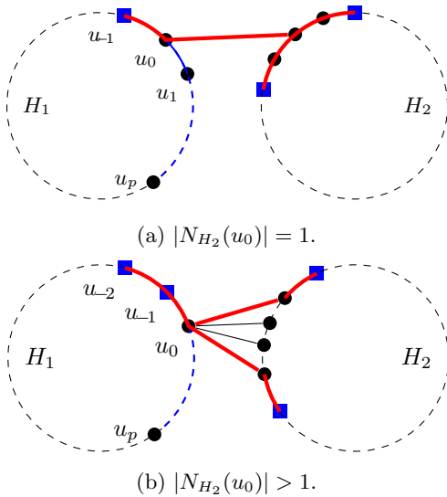
Figure 3: Adjacency of non-congenial holes ( u_{-1} \not\sim H_2 )
