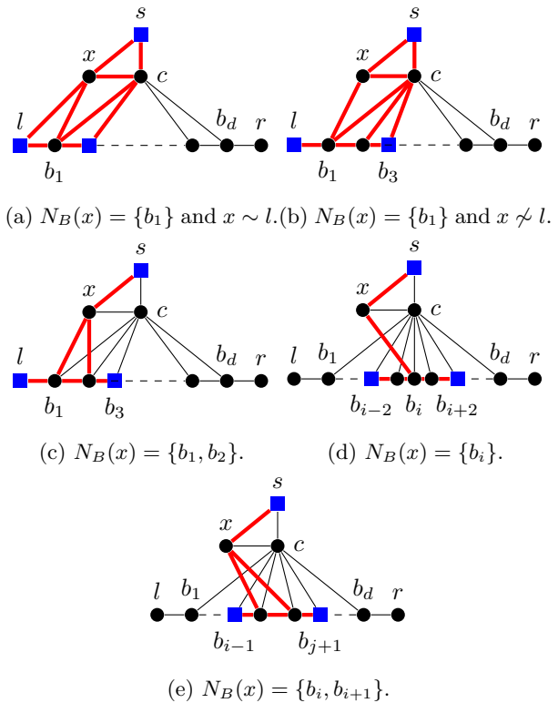
Figure 8: Vertex x in category “partial” [Lem. 5.2].
