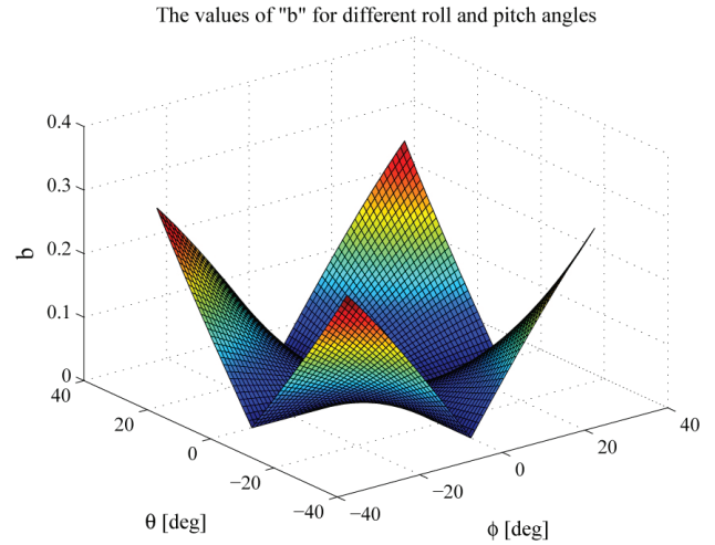
Fig. 7. 'b' parameter values against pitch and bank angles
